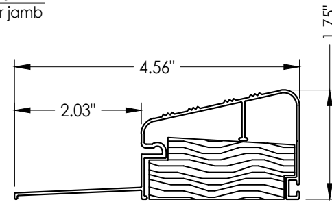
29 OUTSWING THRESHOLD BY DLP
