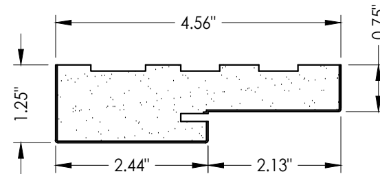
21 HEAD & SIDE Poly fiber jamb
