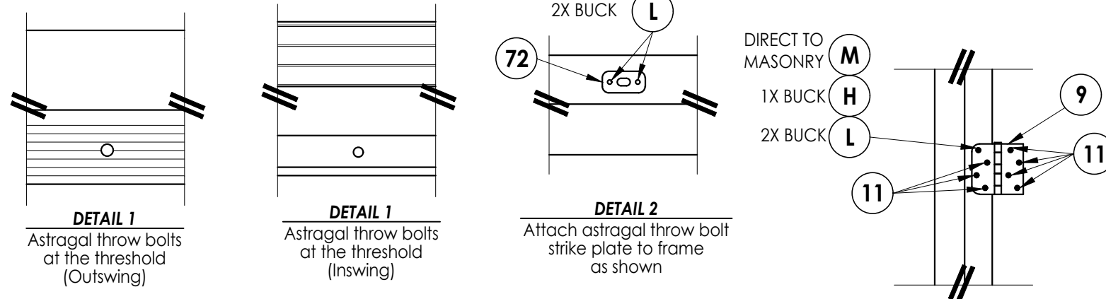
HINGE DETAIL
